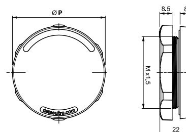
Dimensions [mm]
