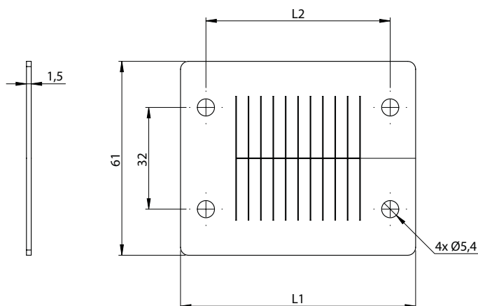
Dimensions (mm)
